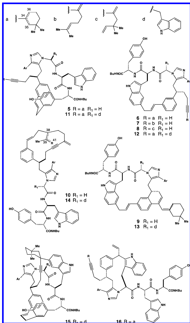
Figure 2. Products derived from processing G-W-Y and W-W-Y independently with reagent 2 , using the chemistry depicted in Figure 1B followed by treatment with MsOH in anhydrous MeNO 2 . Ar = p-F-phenyl. \Delta 38,39 (R = Me) and \Delta 39,41 (R = CH 2 ) isomers of cyclophane 10 characterized separately. 14 observed in \Delta 38,39 form only. Where present, the alkynyl cyclohexene motif (a) is isolated as a mixture of \Delta 34,35 and \Delta 34,36 olefin isomers.
